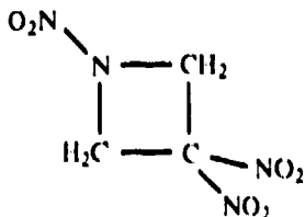
FIGURE 1. Chemical structure of TNAZ, C 2 H 3 N 2 O 6 .
